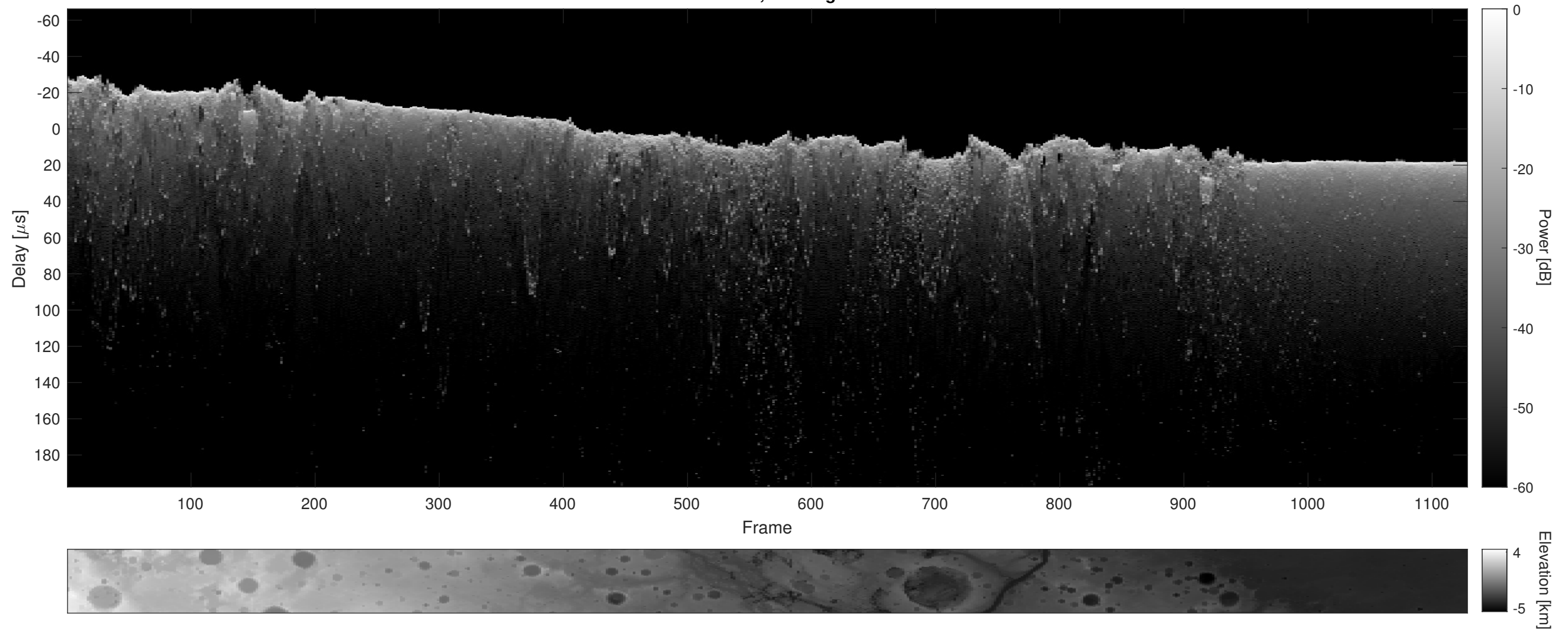
Orbit 22932, Cluttergram
