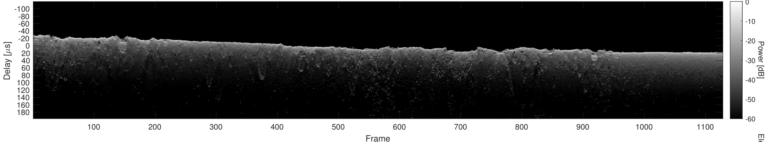
Orbit 22932, Cluttergram
