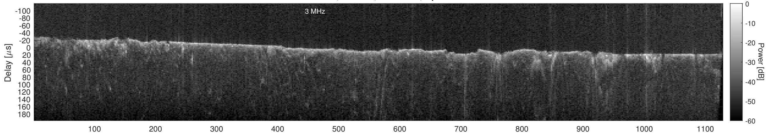
Orbit 22932, Cluttergram
