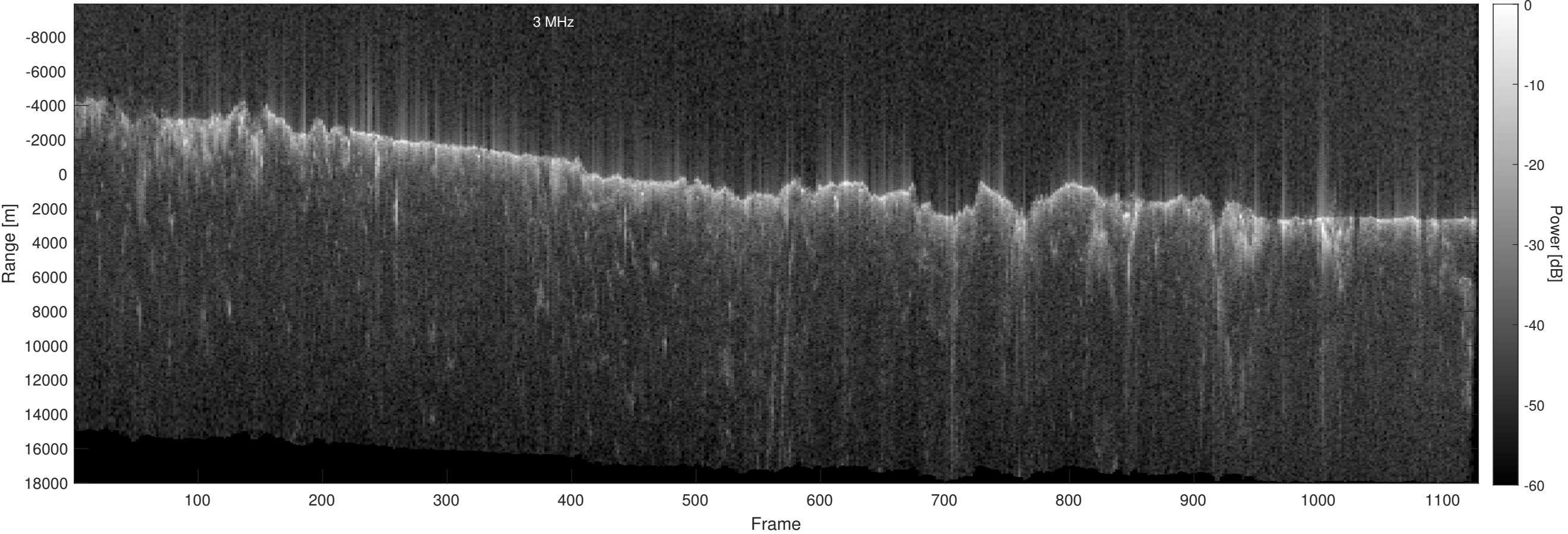
Orbit 22932, Optimized, No Window, Depth-Corrected, Channel 2
