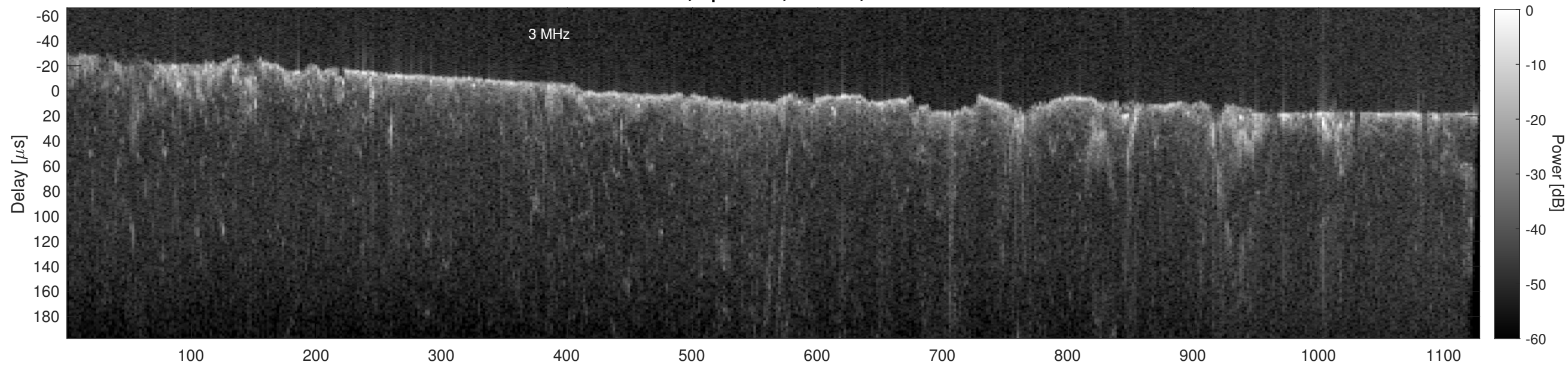
Orbit 22932, Cluttergram
