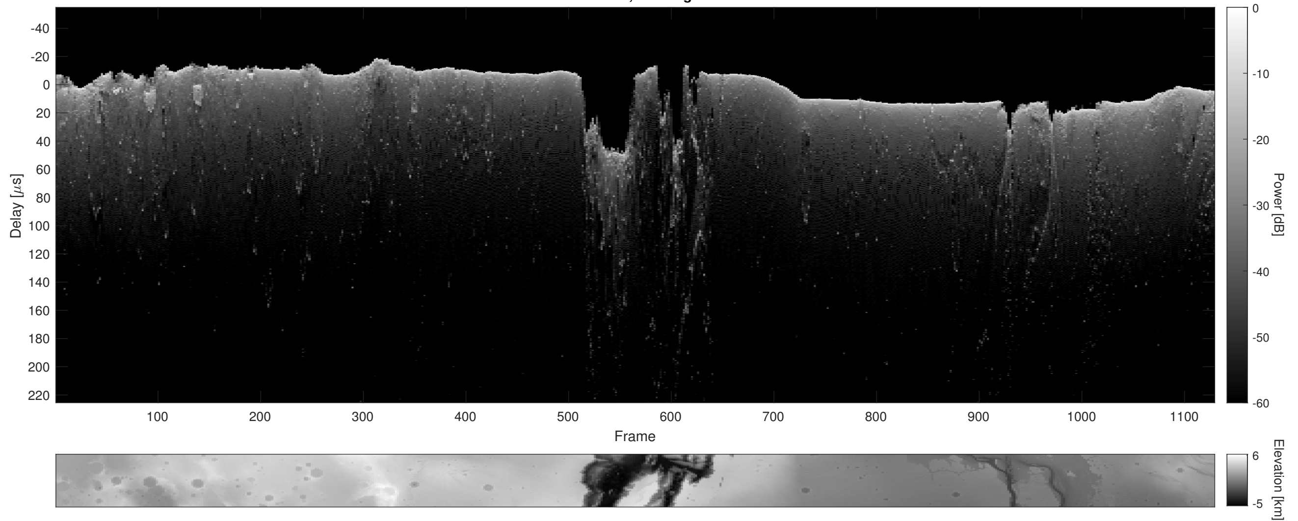
Orbit 22936, Cluttergram
