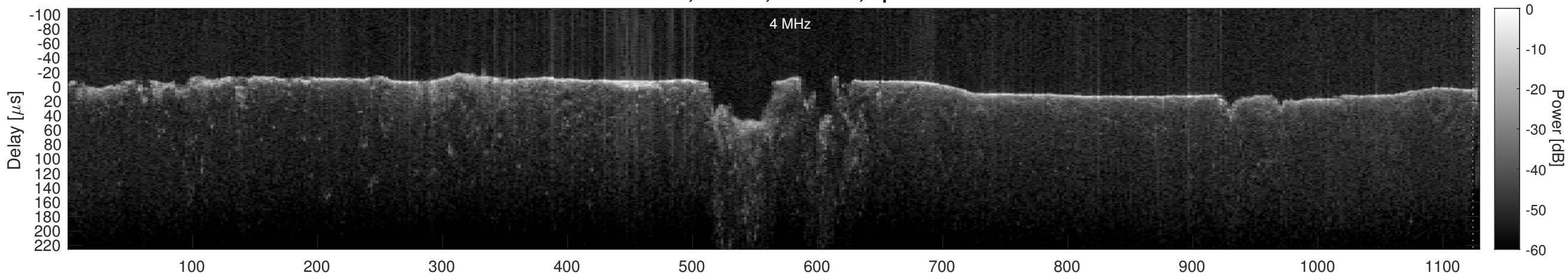
Orbit 22936, Cluttergram
