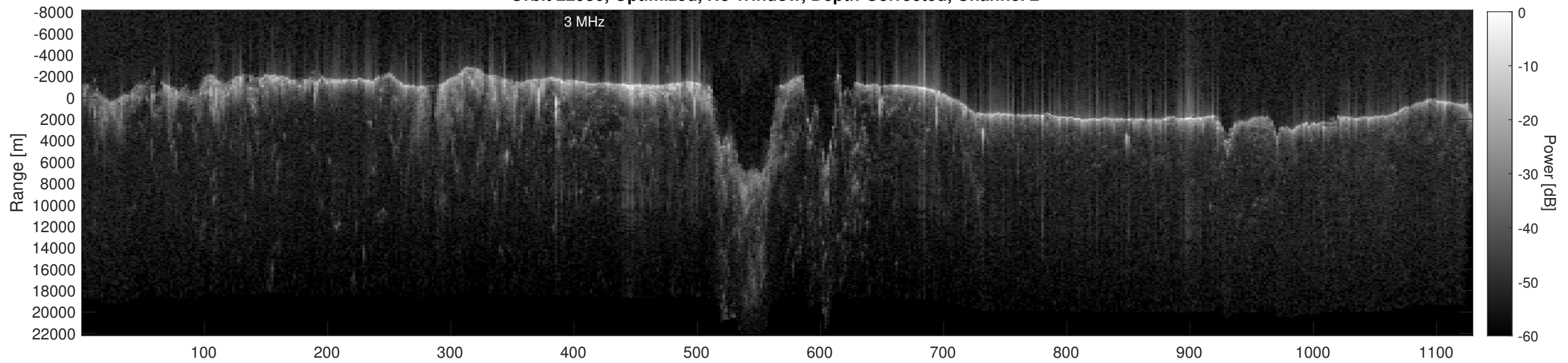
Orbit 22936, Depth-Corrected Cluttergram
