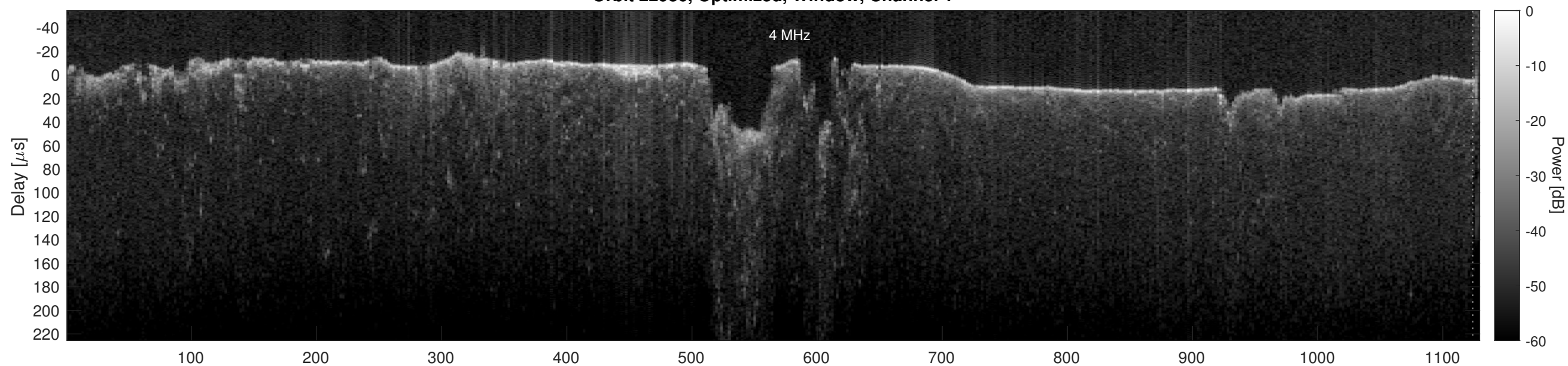
Orbit 22936, Optimized, Window, Channel 2
