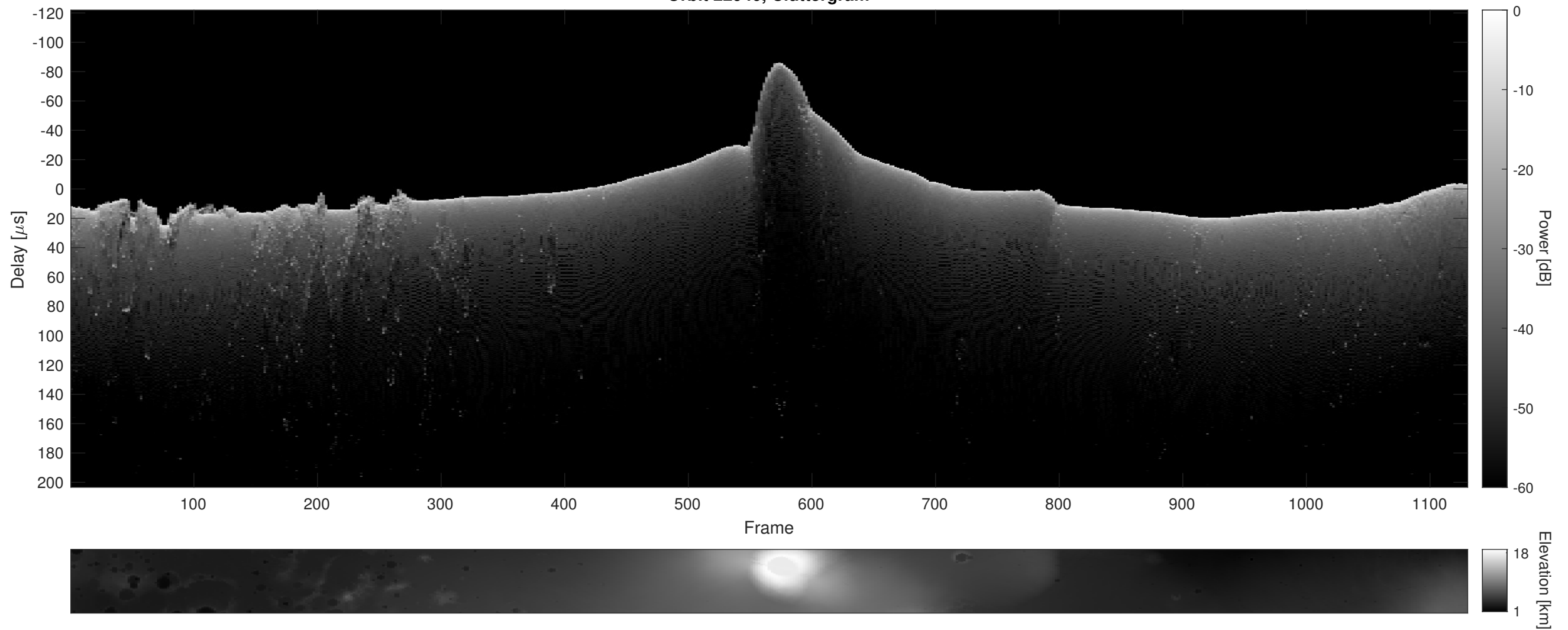
Orbit 22940, Cluttergram
