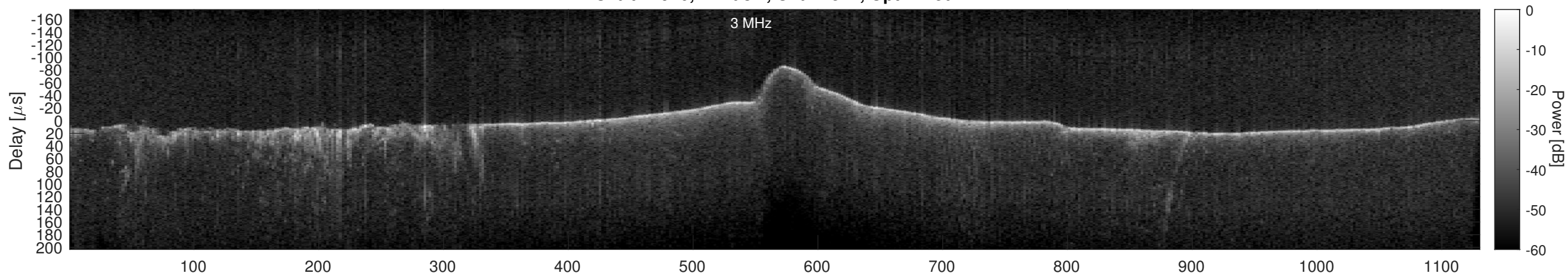
Orbit 22940, Cluttergram
