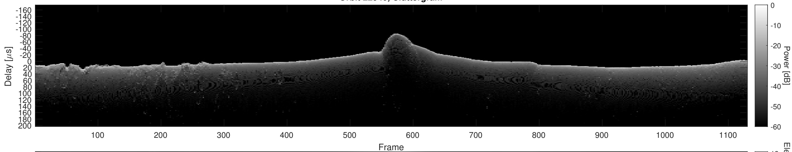
Orbit 22940, Cluttergram
