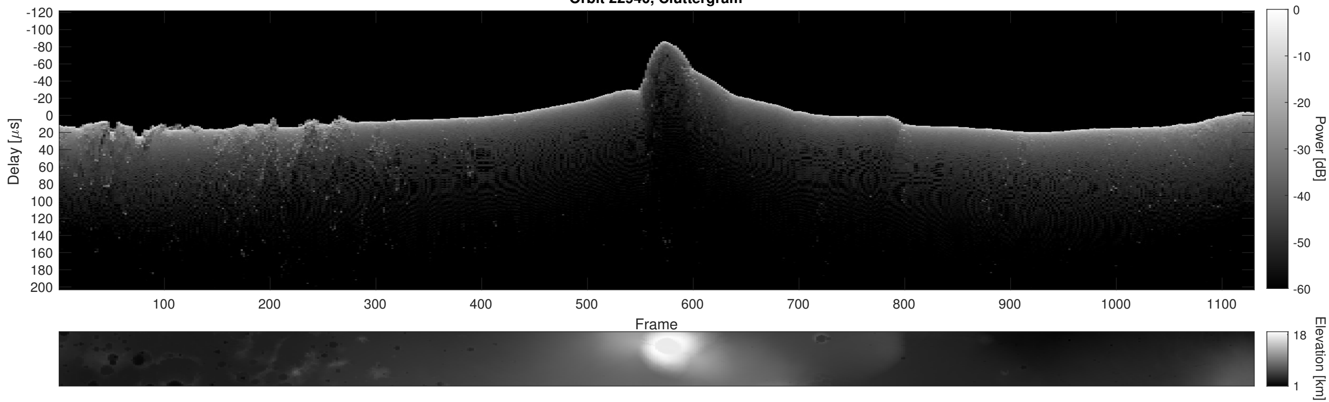
Orbit 22940, Cluttergram
