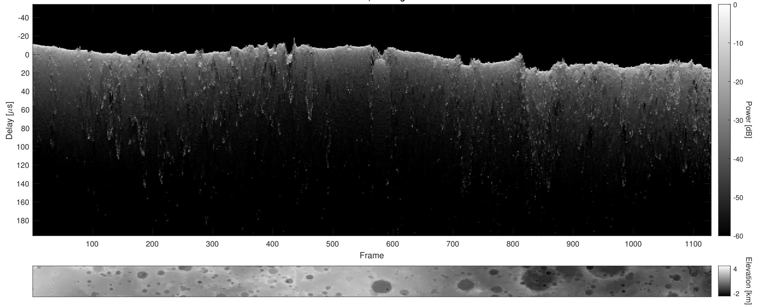
Orbit 22942, Cluttergram
