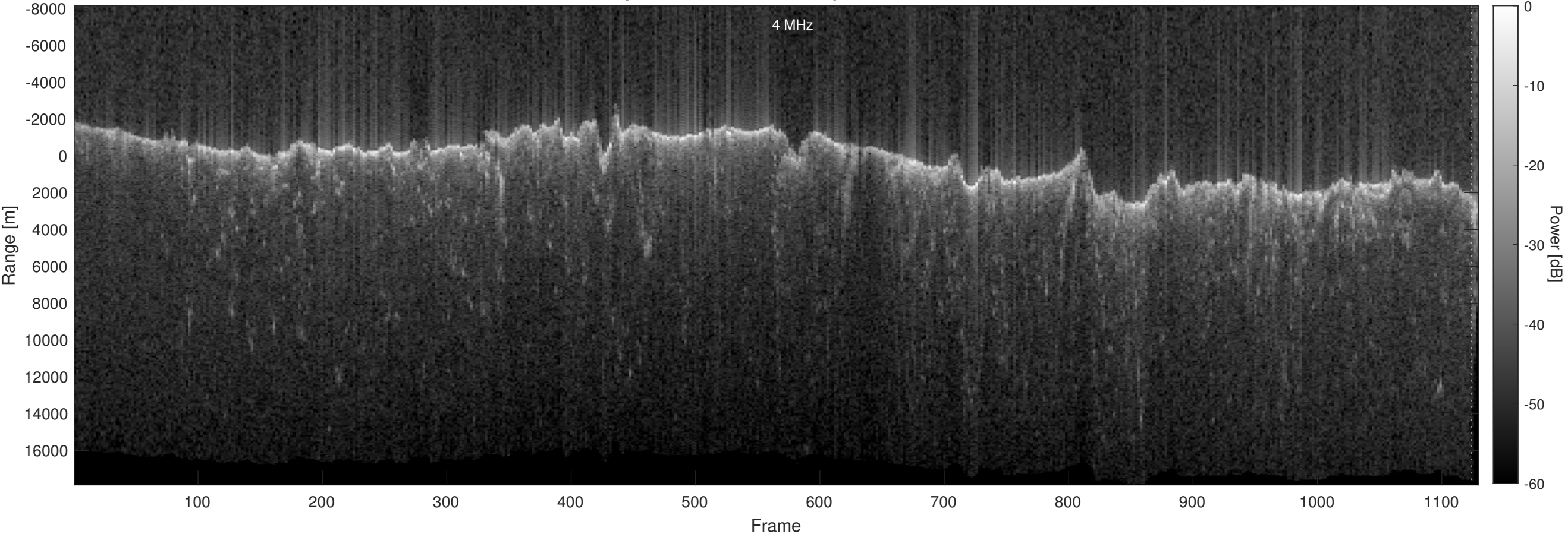
Orbit 22942, Optimized, No Window, Depth-Corrected, Channel 2
