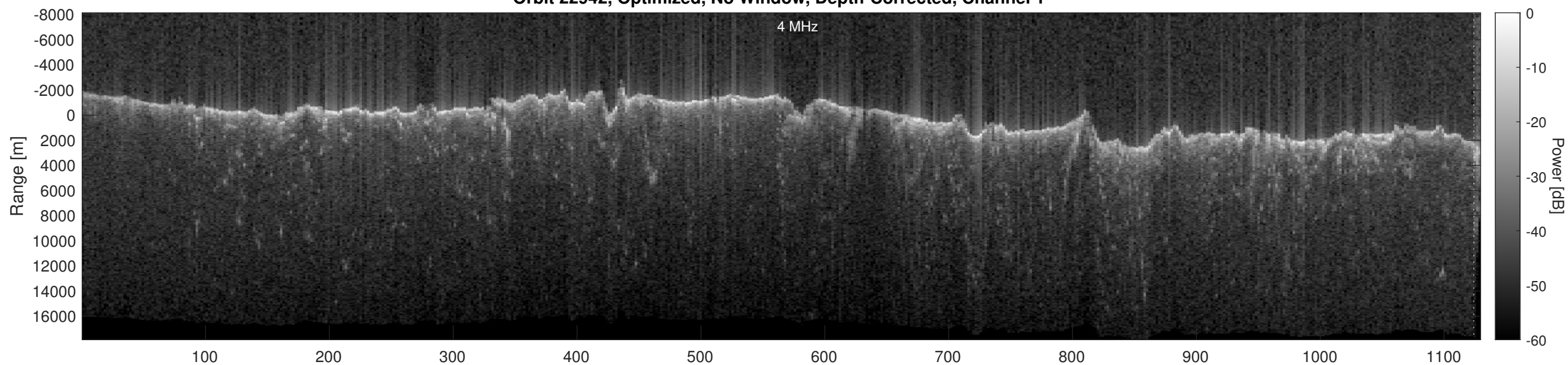
Orbit 22942, Optimized, No Window, Depth-Corrected, Channel 2
