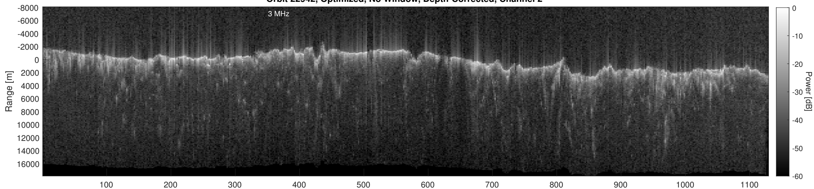
Orbit 22942, Depth-Corrected Cluttergram
