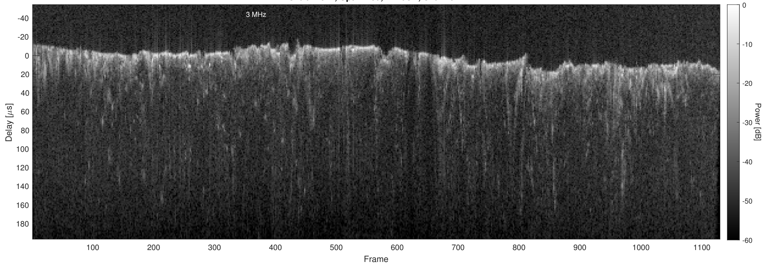
Orbit 22942, Optimized, Window, Channel 2
