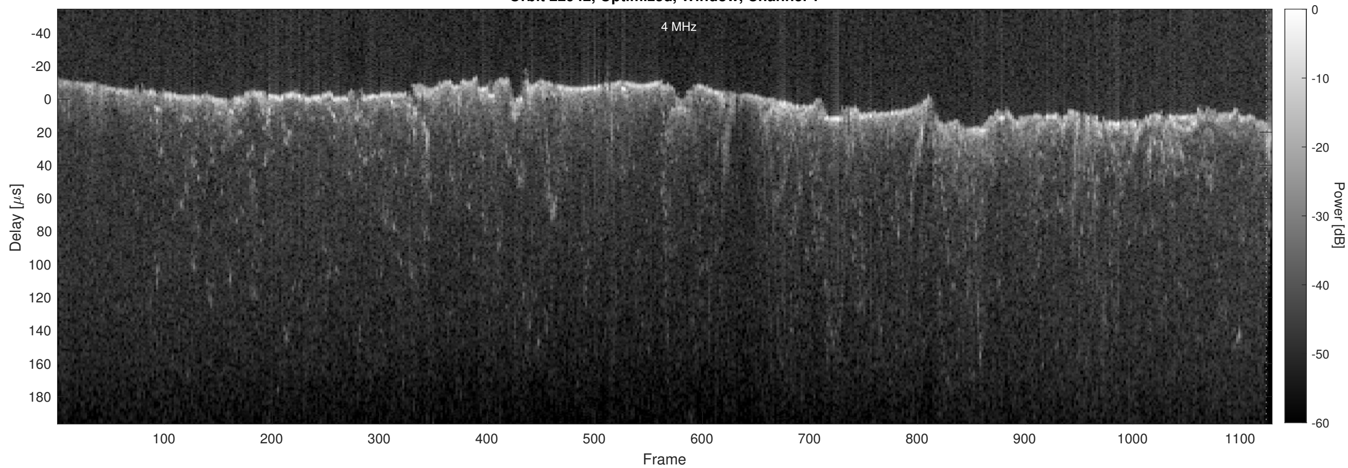
Orbit 22942, Optimized, Window, Channel 2
