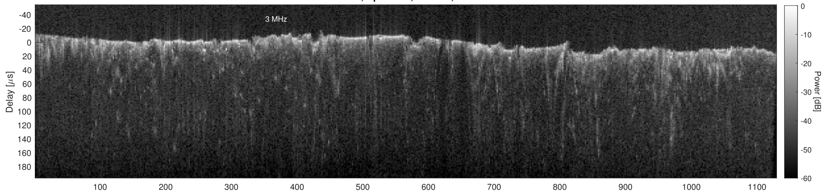
Orbit 22942, Cluttergram
