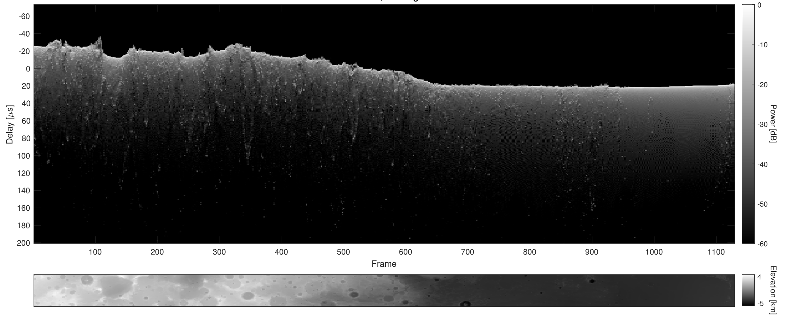
Orbit 22944, Cluttergram
