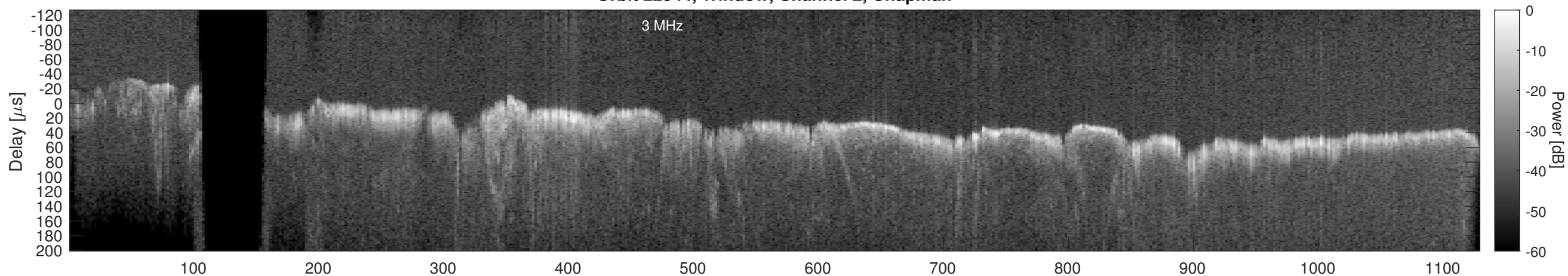
Orbit 22944, Window, Channel 2, Optimized
