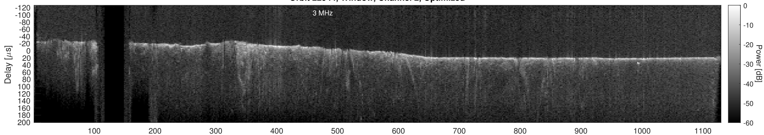
Orbit 22944, Cluttergram
