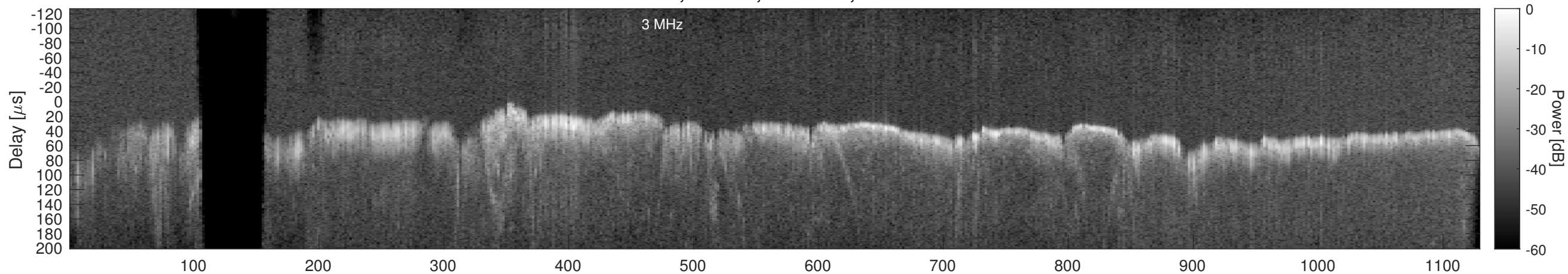
Orbit 22944, Window, Channel 2, Chapman
