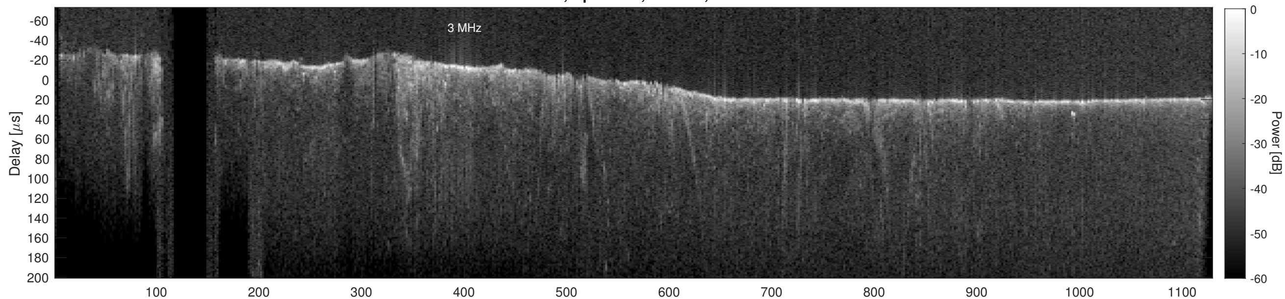
Orbit 22944, Cluttergram
