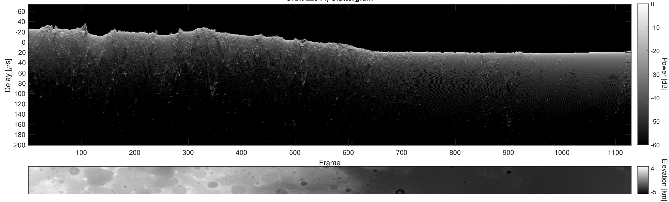
Orbit 22944, Cluttergram
