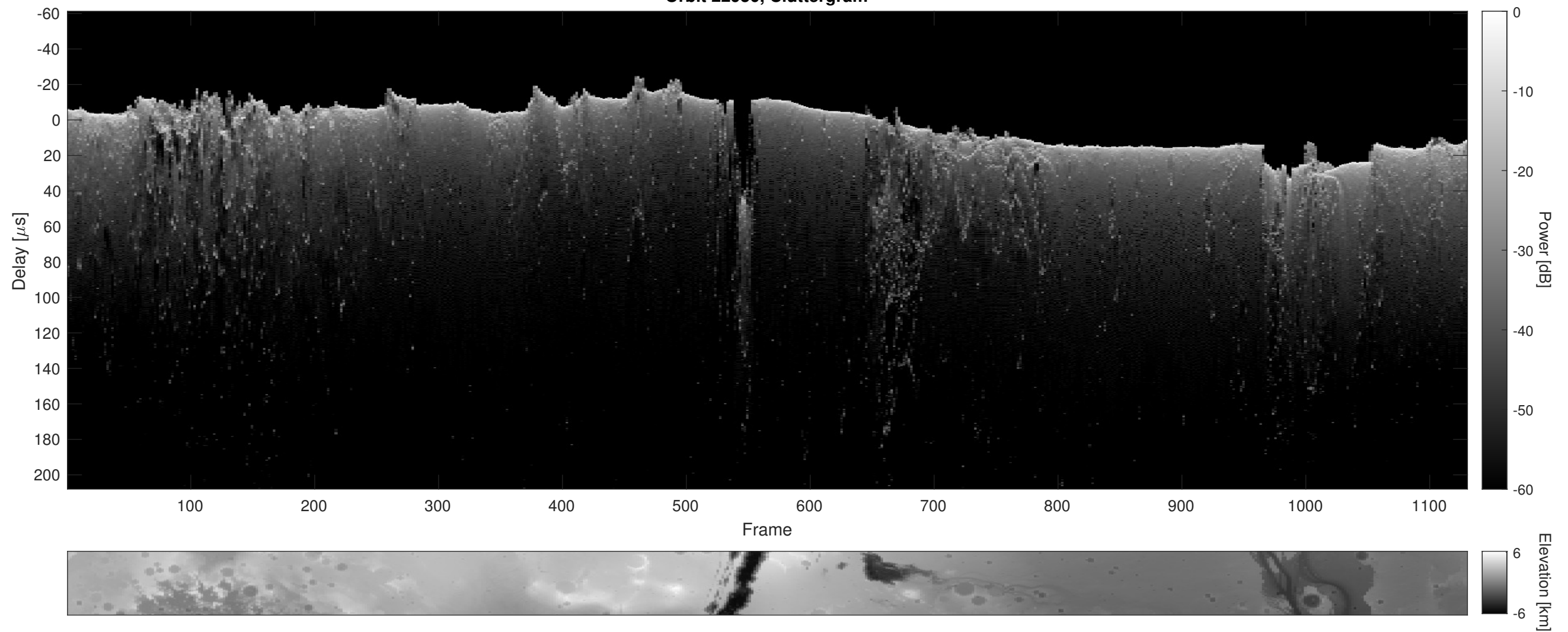
Orbit 22950, Cluttergram
