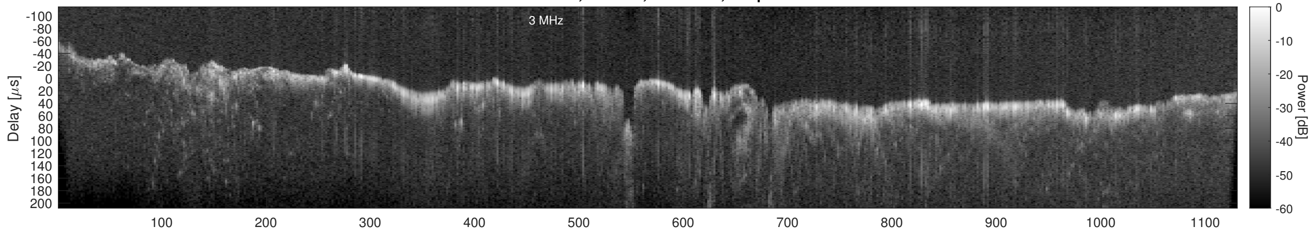
Orbit 22950, Window, Channel 2, Optimized
