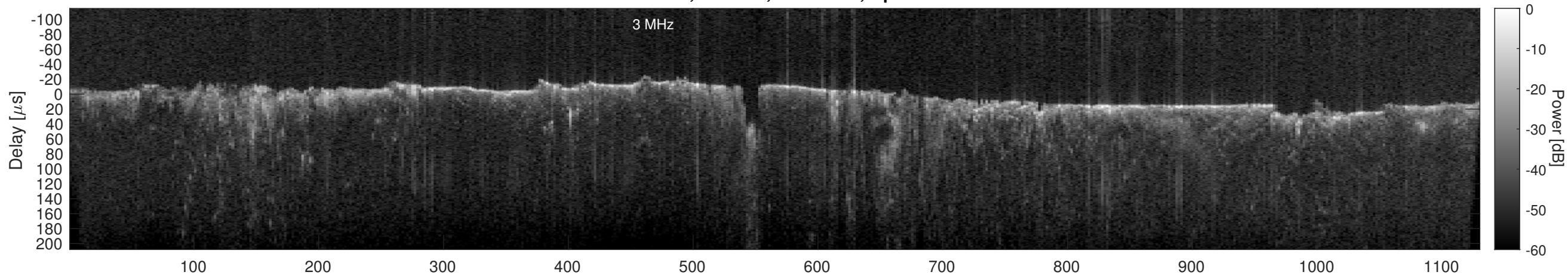
Orbit 22950, Cluttergram
