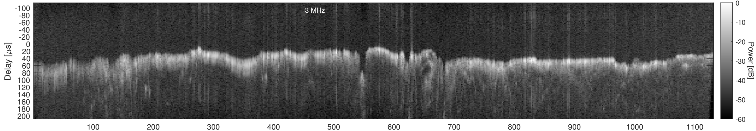
Orbit 22950, Window, Channel 2, Chapman
