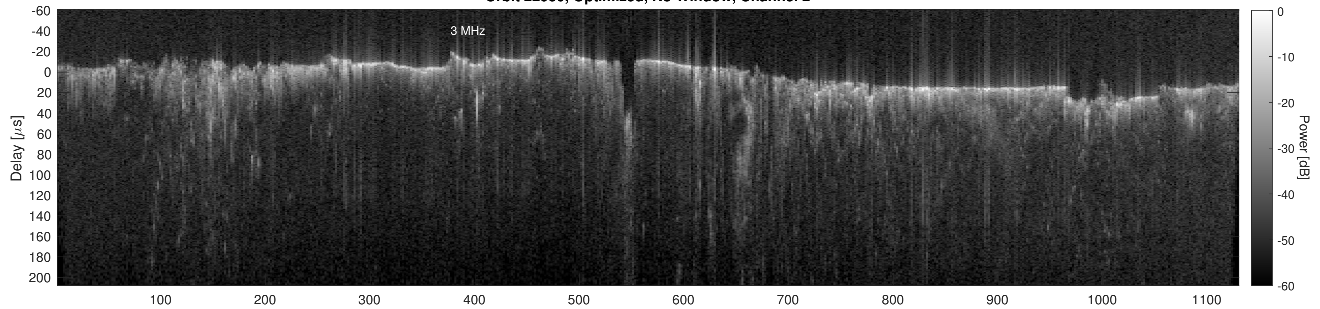
Orbit 22950, Cluttergram
