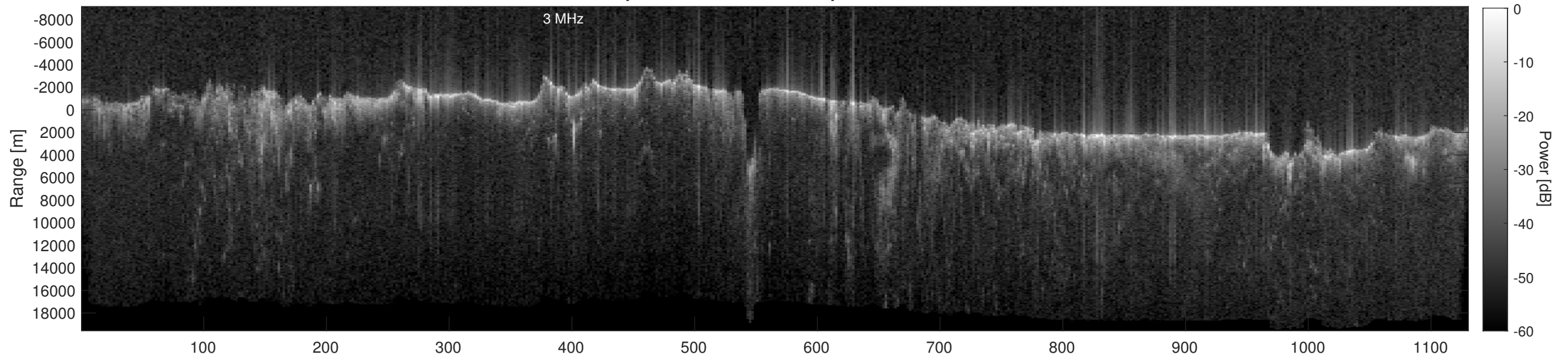
Orbit 22950, Depth-Corrected Cluttergram
