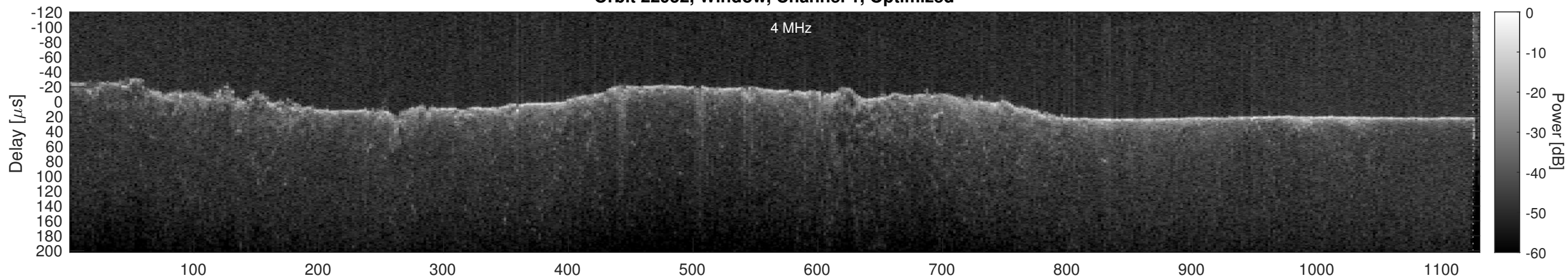
Orbit 22952, Cluttergram
