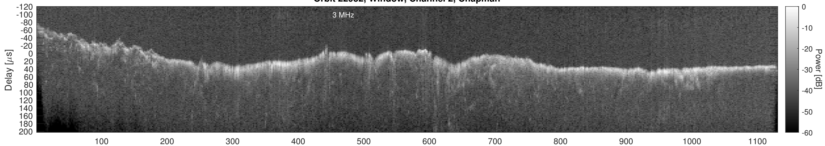
Orbit 22952, Window, Channel 2, Optimized
