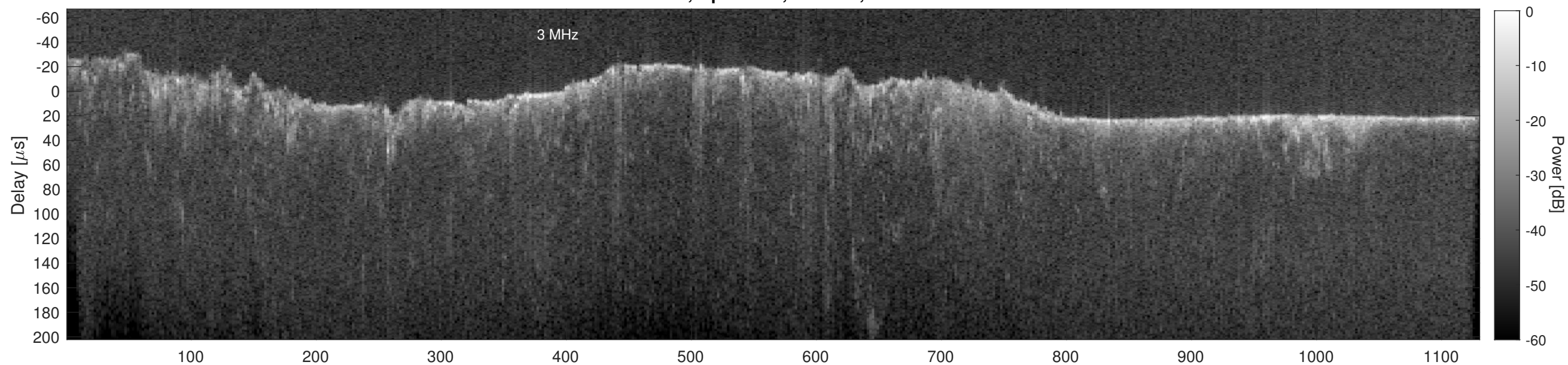
Orbit 22952, Cluttergram
