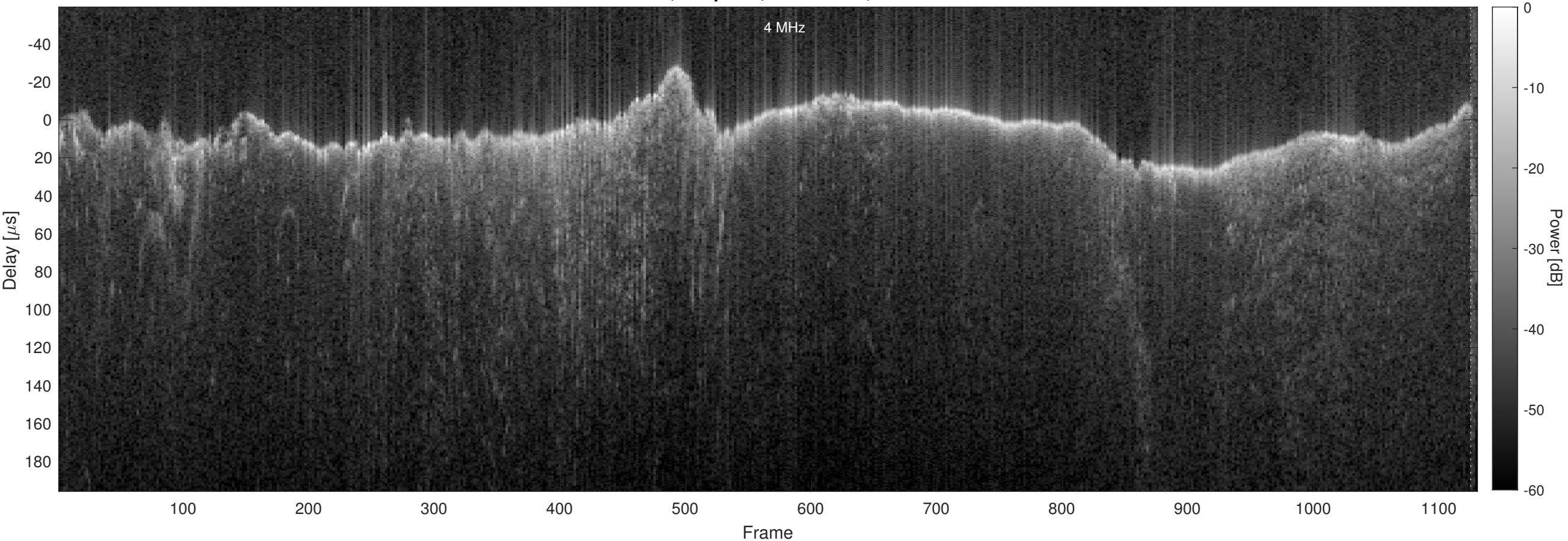
Orbit 22954, Chapman, No Window, Channel 2
