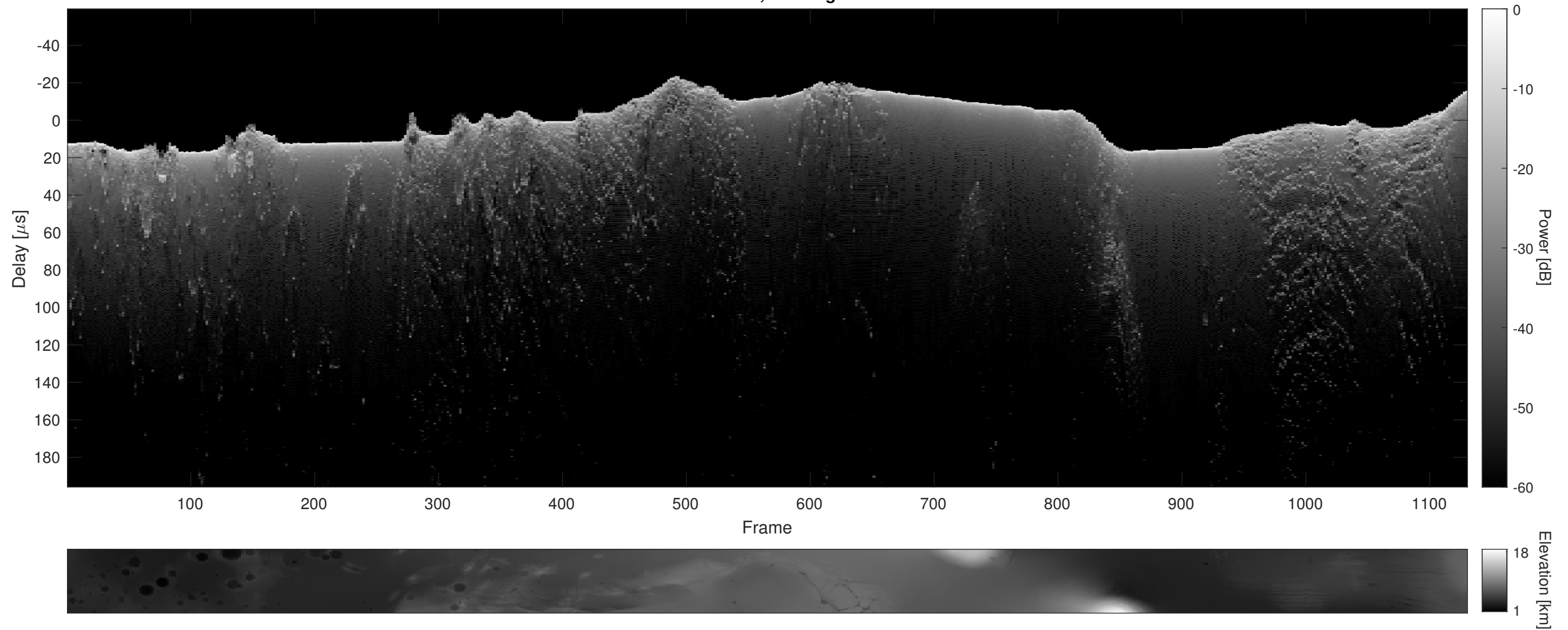
Orbit 22954, Cluttergram
