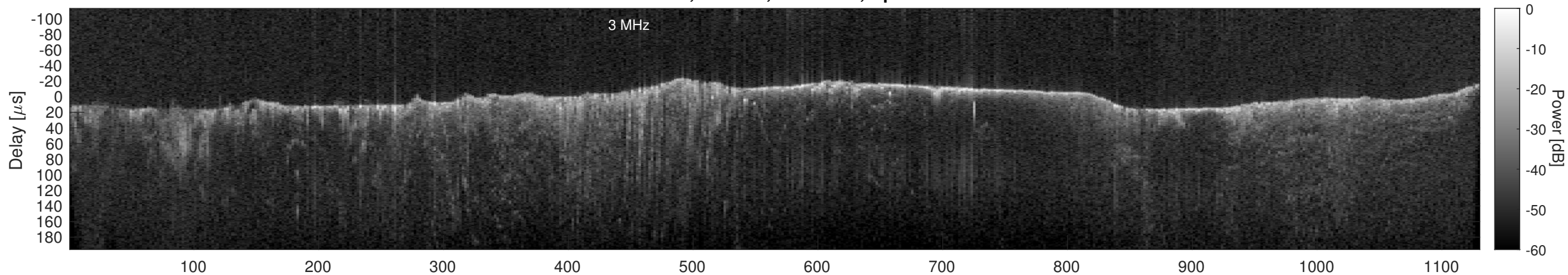
Orbit 22954, Cluttergram
