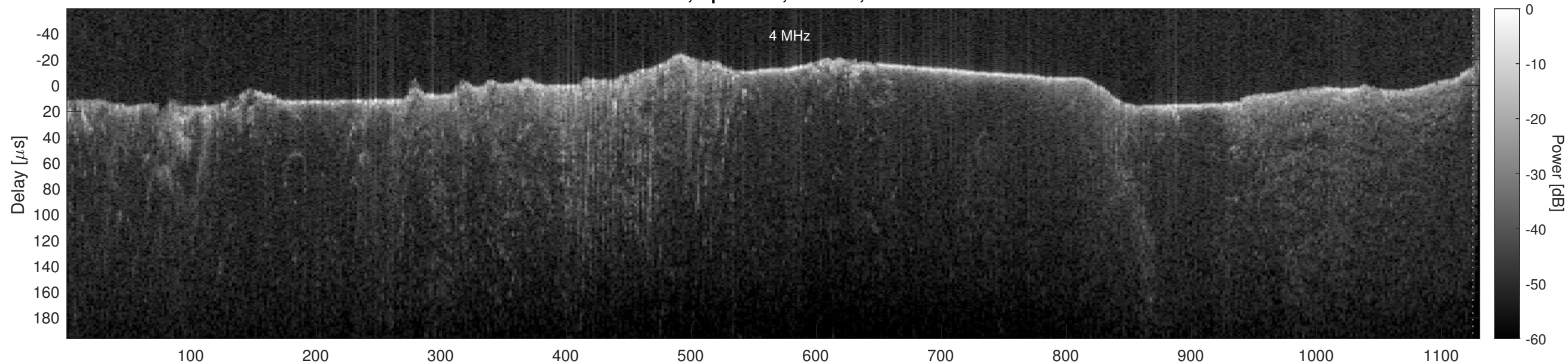
Orbit 22954, Optimized, Window, Channel 2
