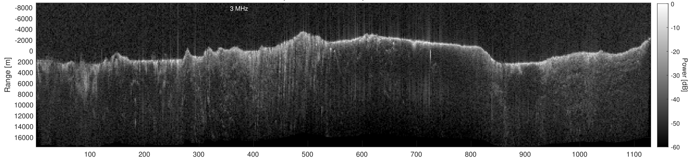
Orbit 22954, Depth-Corrected Cluttergram
