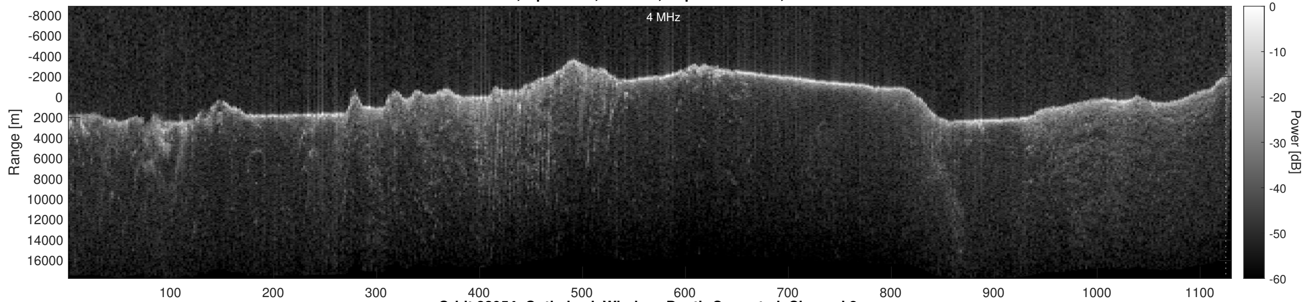
Orbit 22954, Optimized, Window, Depth-Corrected, Channel 2
