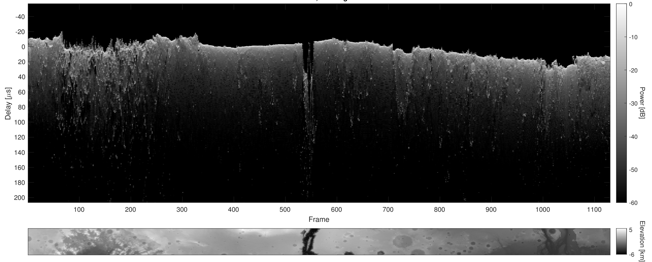
Orbit 22957, Cluttergram
