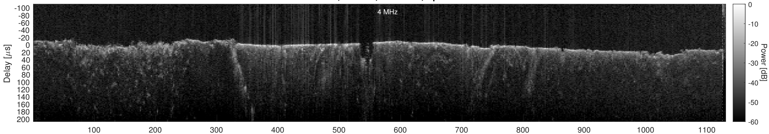
Orbit 22957, Cluttergram
