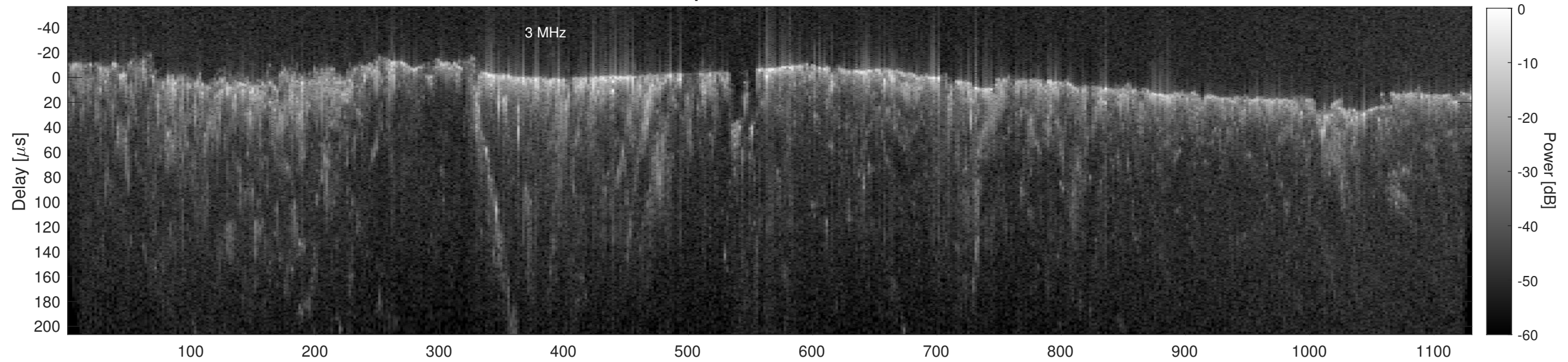
Orbit 22957, Cluttergram
