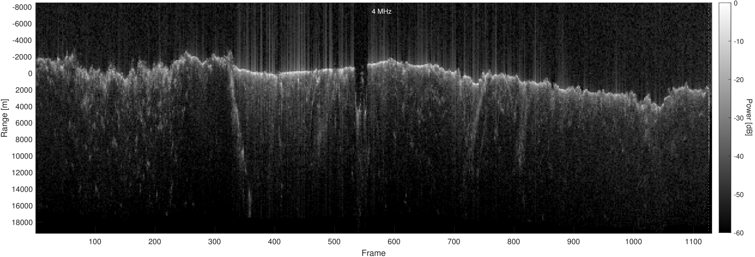
Orbit 22957, Optimized, No Window, Depth-Corrected, Channel 2
