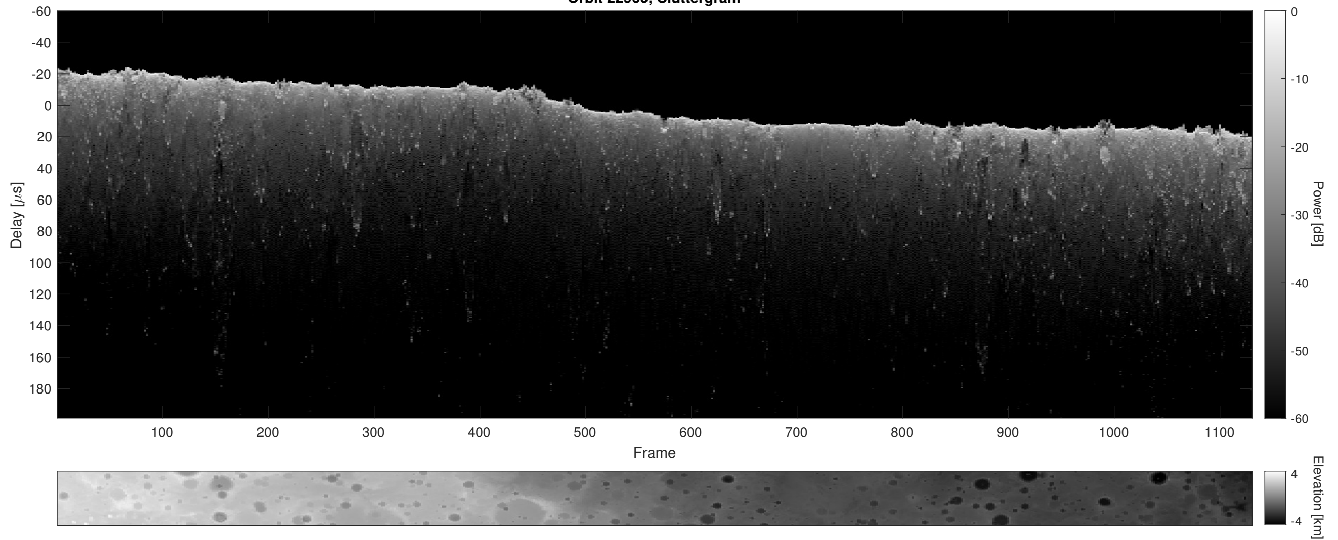
Orbit 22960, Cluttergram
