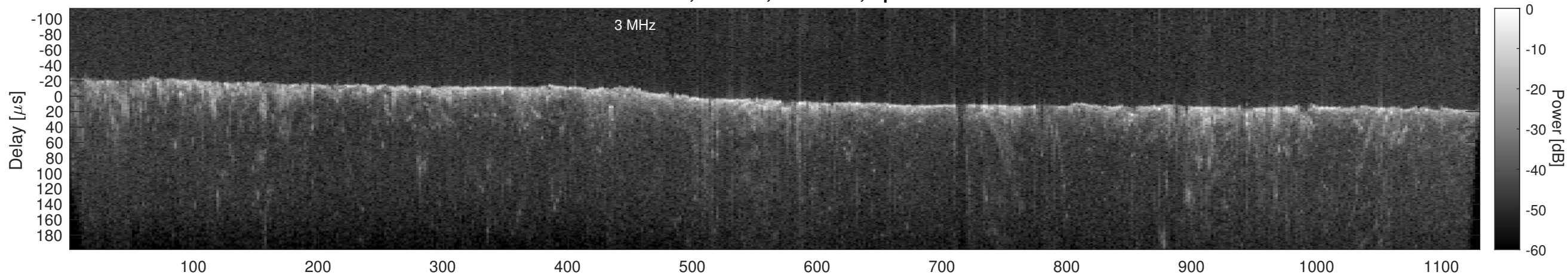
Orbit 22960, Cluttergram
