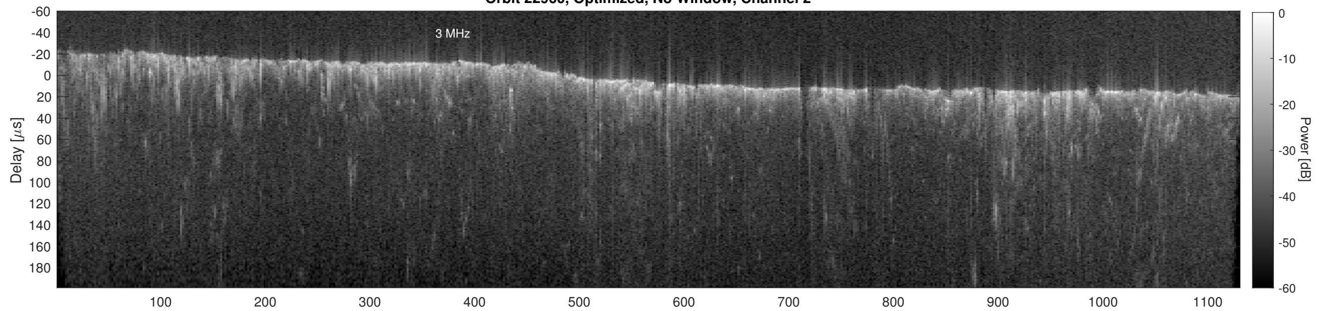
Orbit 22960, Cluttergram
