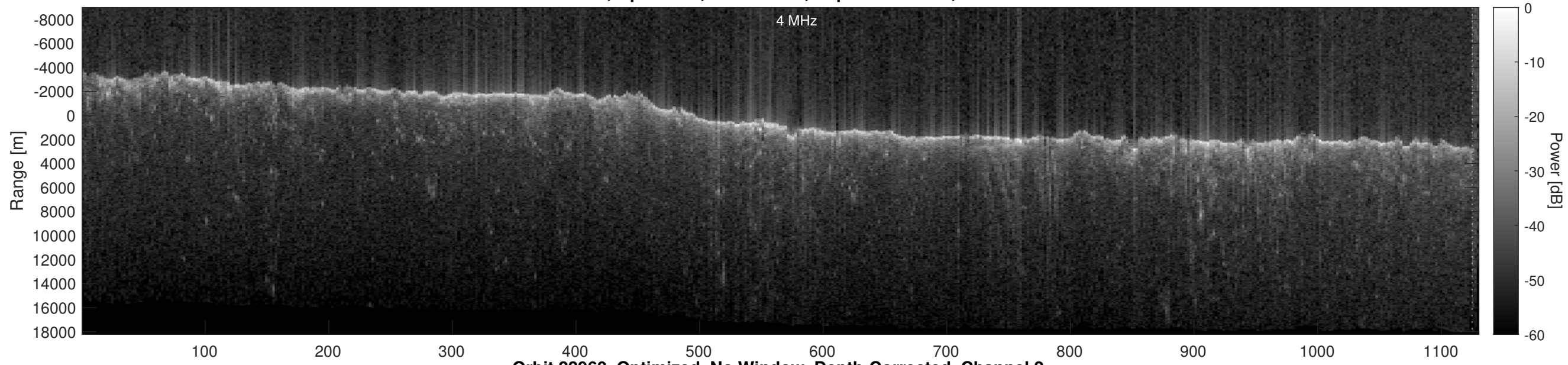
Orbit 22960, Optimized, No Window, Depth-Corrected, Channel 2
