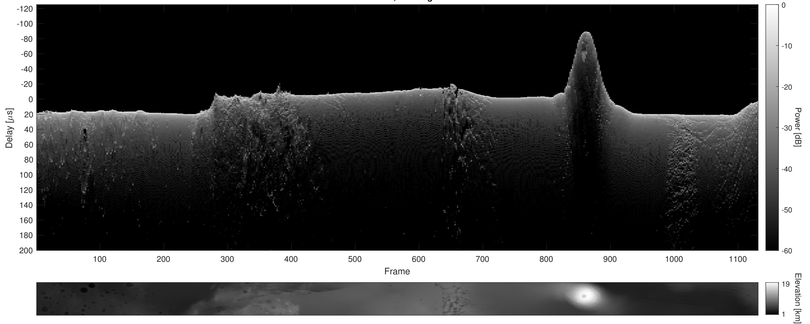
Orbit 22961, Cluttergram
