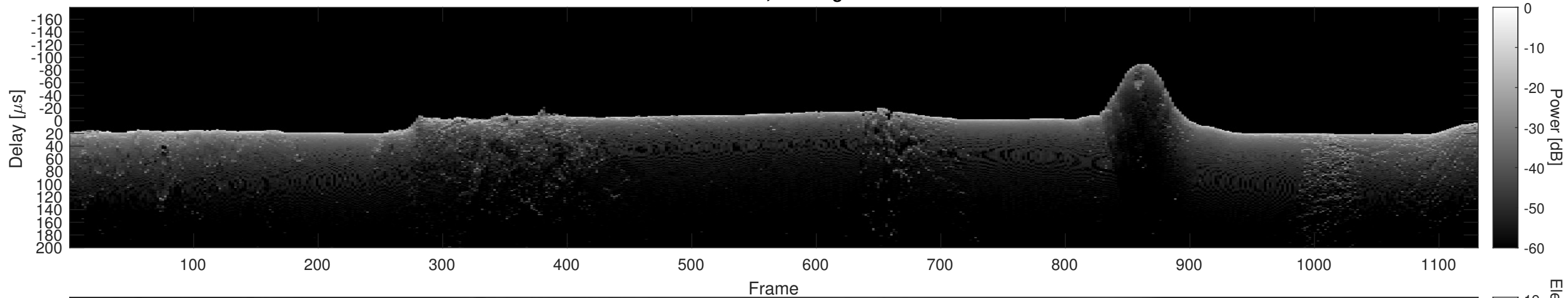
Orbit 22961, Cluttergram
