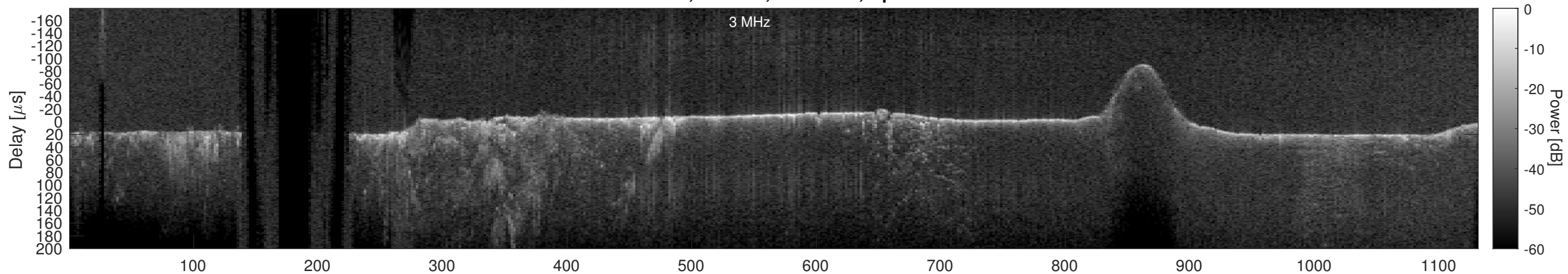
Orbit 22961, Cluttergram
