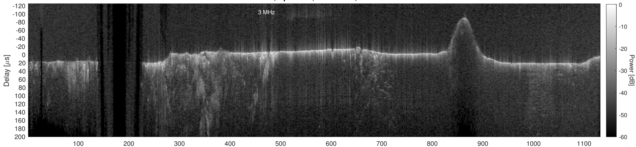
Orbit 22961, Cluttergram
