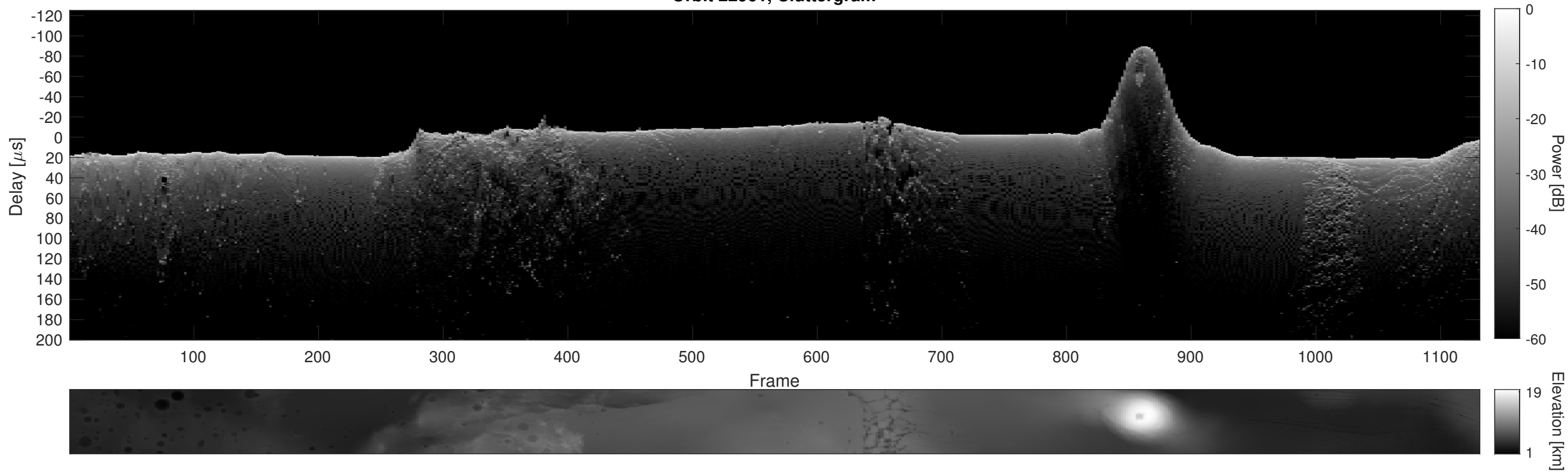
Orbit 22961, Cluttergram
