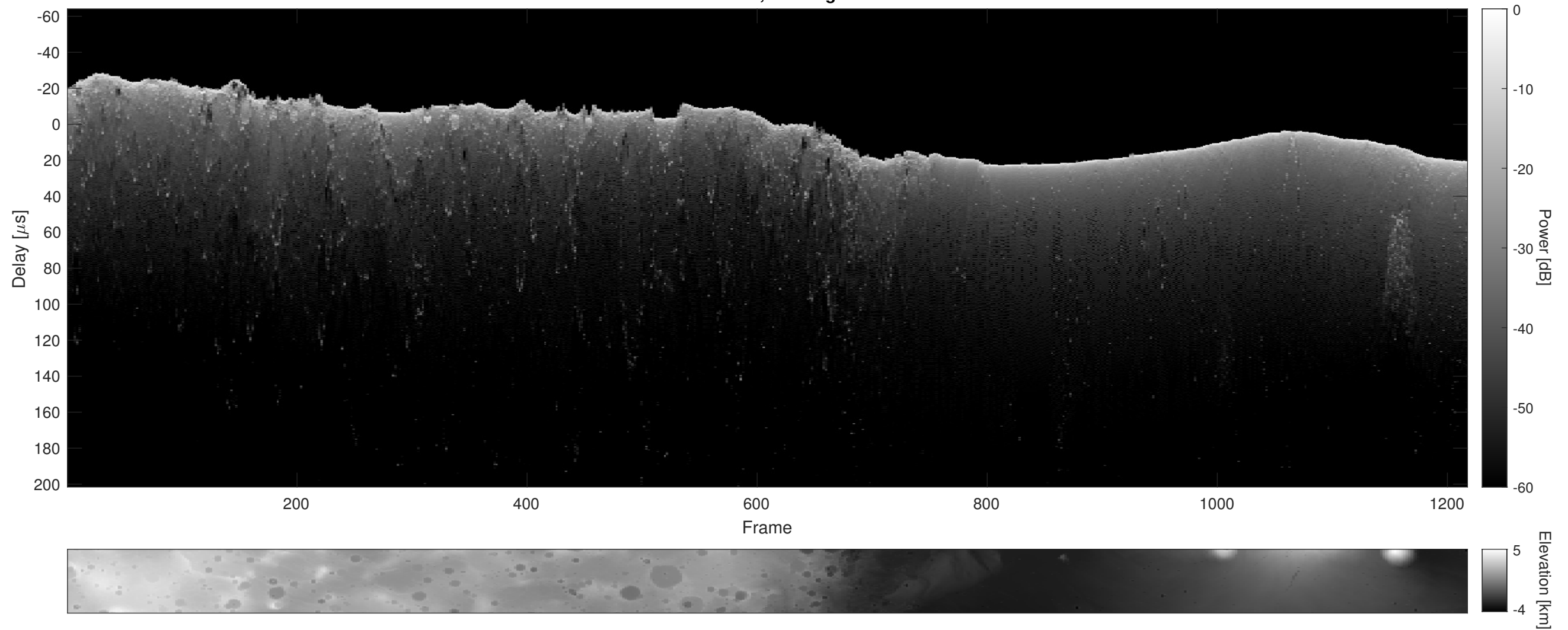
Orbit 22962, Cluttergram
