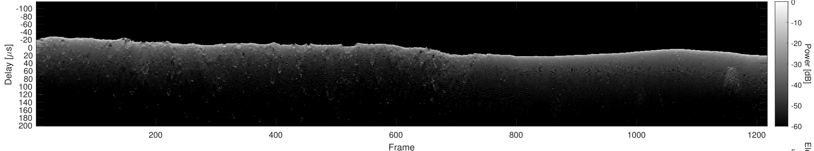
Orbit 22962, Cluttergram
