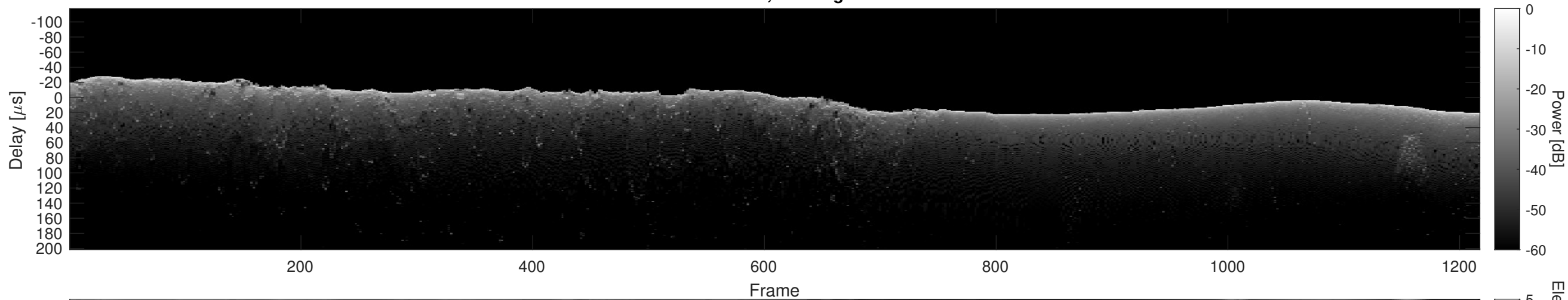
Orbit 22962, Cluttergram
