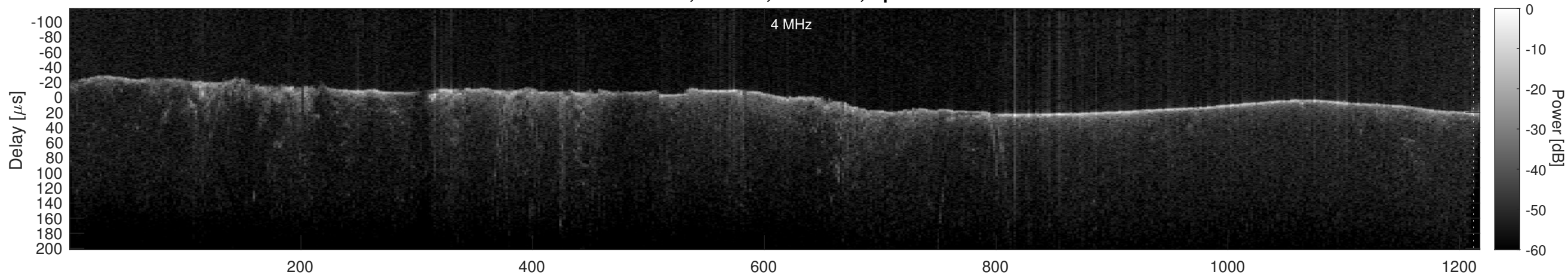
Orbit 22962, Cluttergram
