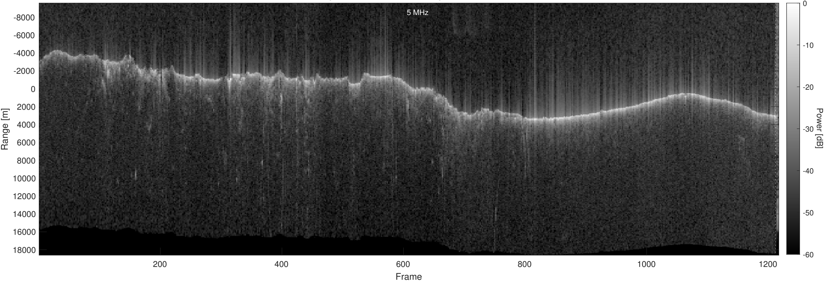
Orbit 22962, Optimized, No Window, Depth-Corrected, Channel 2
