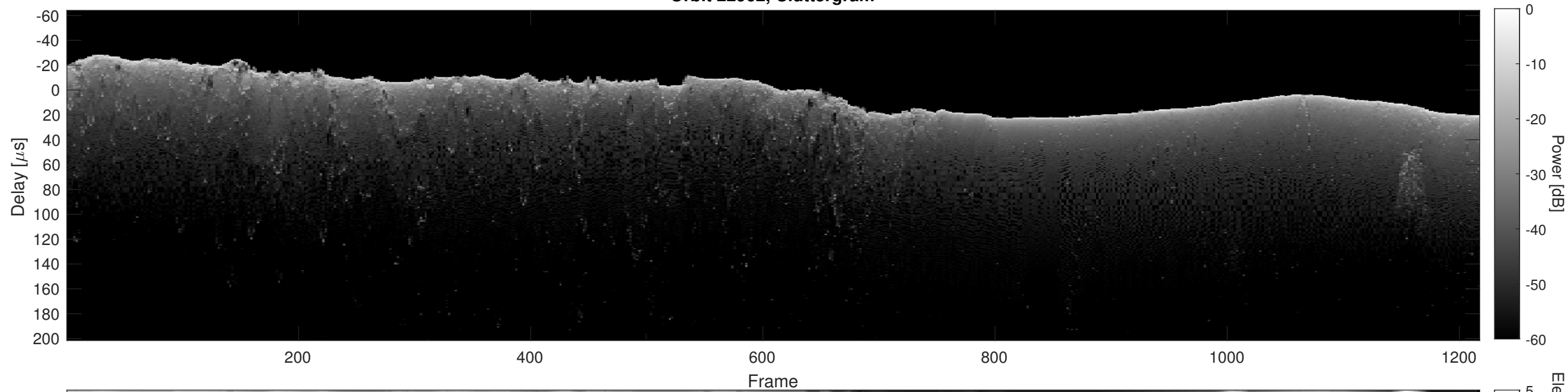
Orbit 22962, Cluttergram
