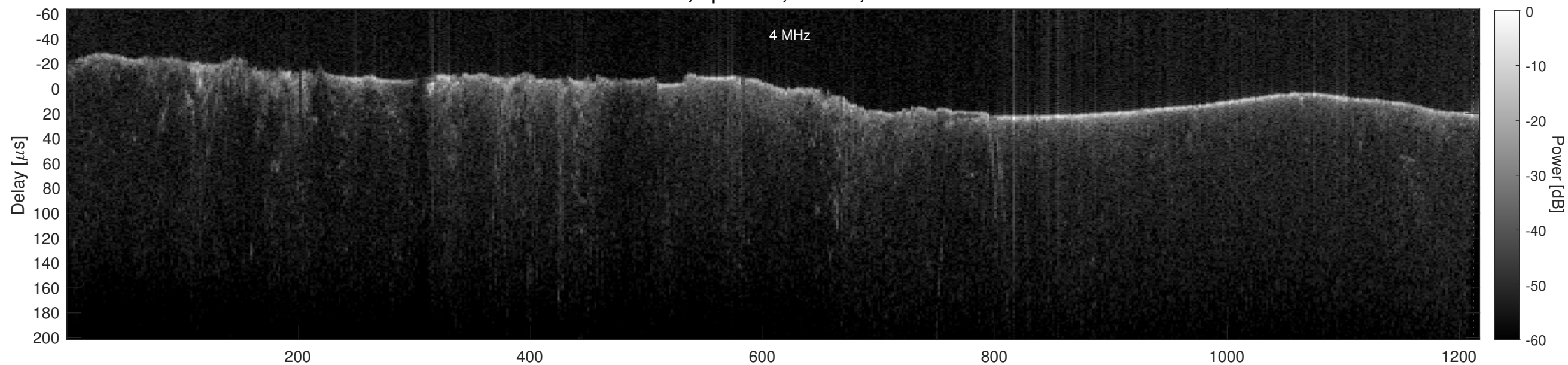
Orbit 22962, Cluttergram
