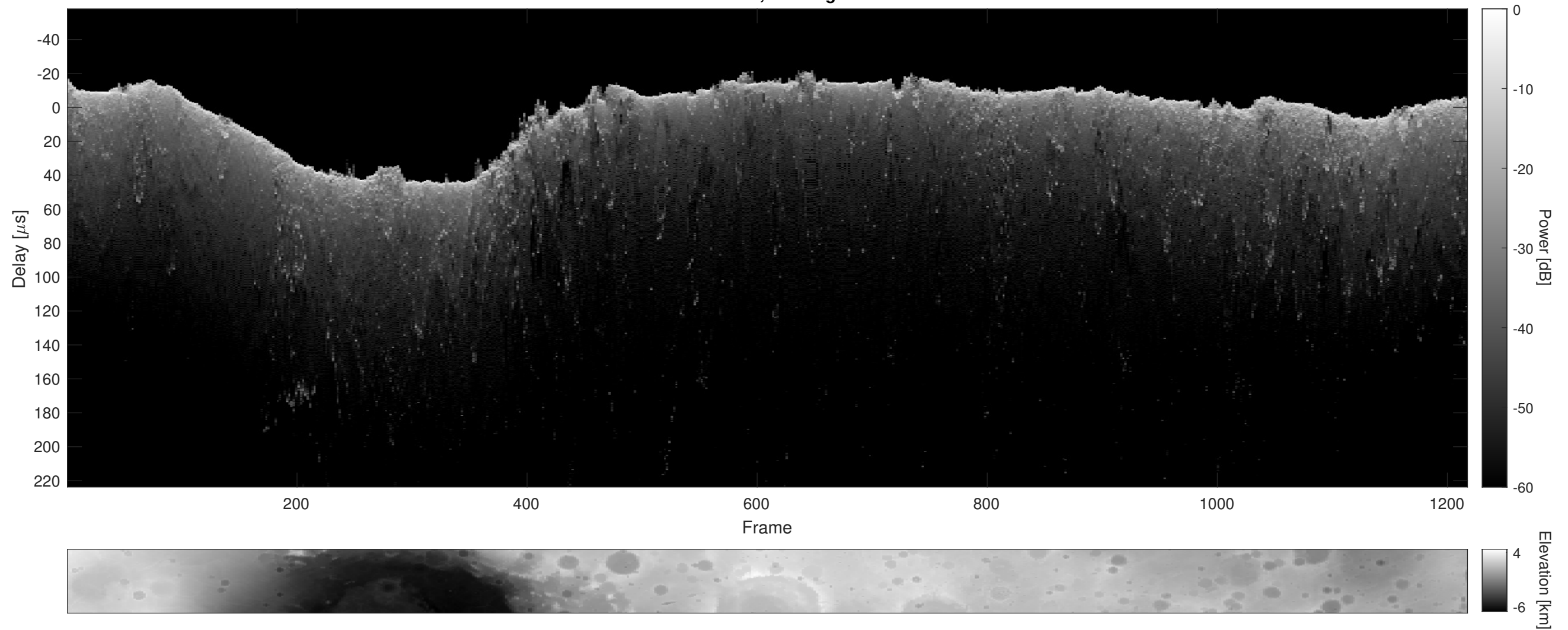
Orbit 22963, Cluttergram
